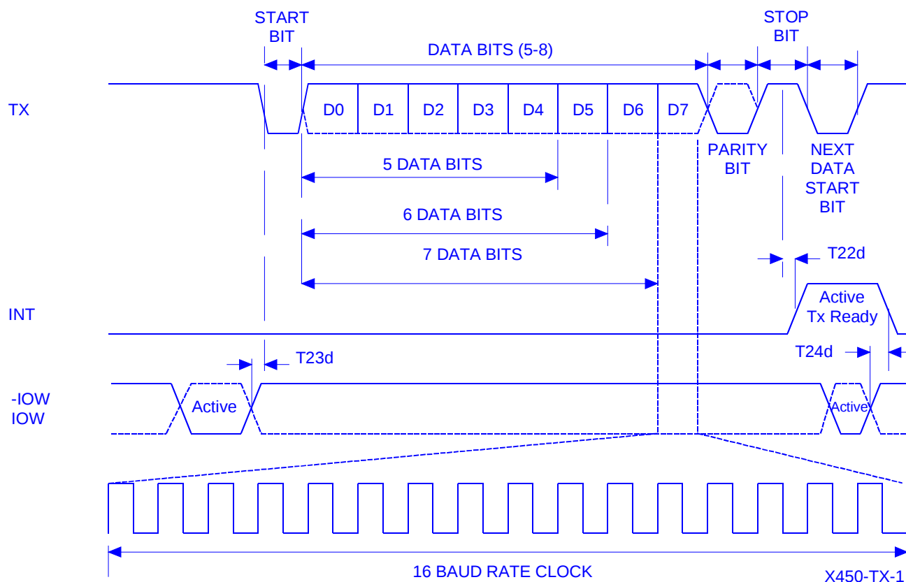
Transmit timing
