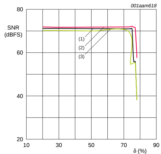
Fig 8. Signal-to-noise ratio as a function of duty cycle ( \delta )
