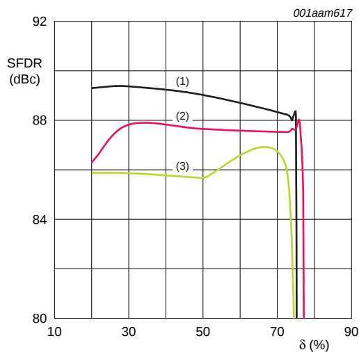
Fig 7. Spurious-free dynamic range as a function of duty cycle ( \delta )
