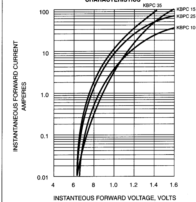
FIG. 3-TYPICAL FORWARD CHARACTERISTICS
