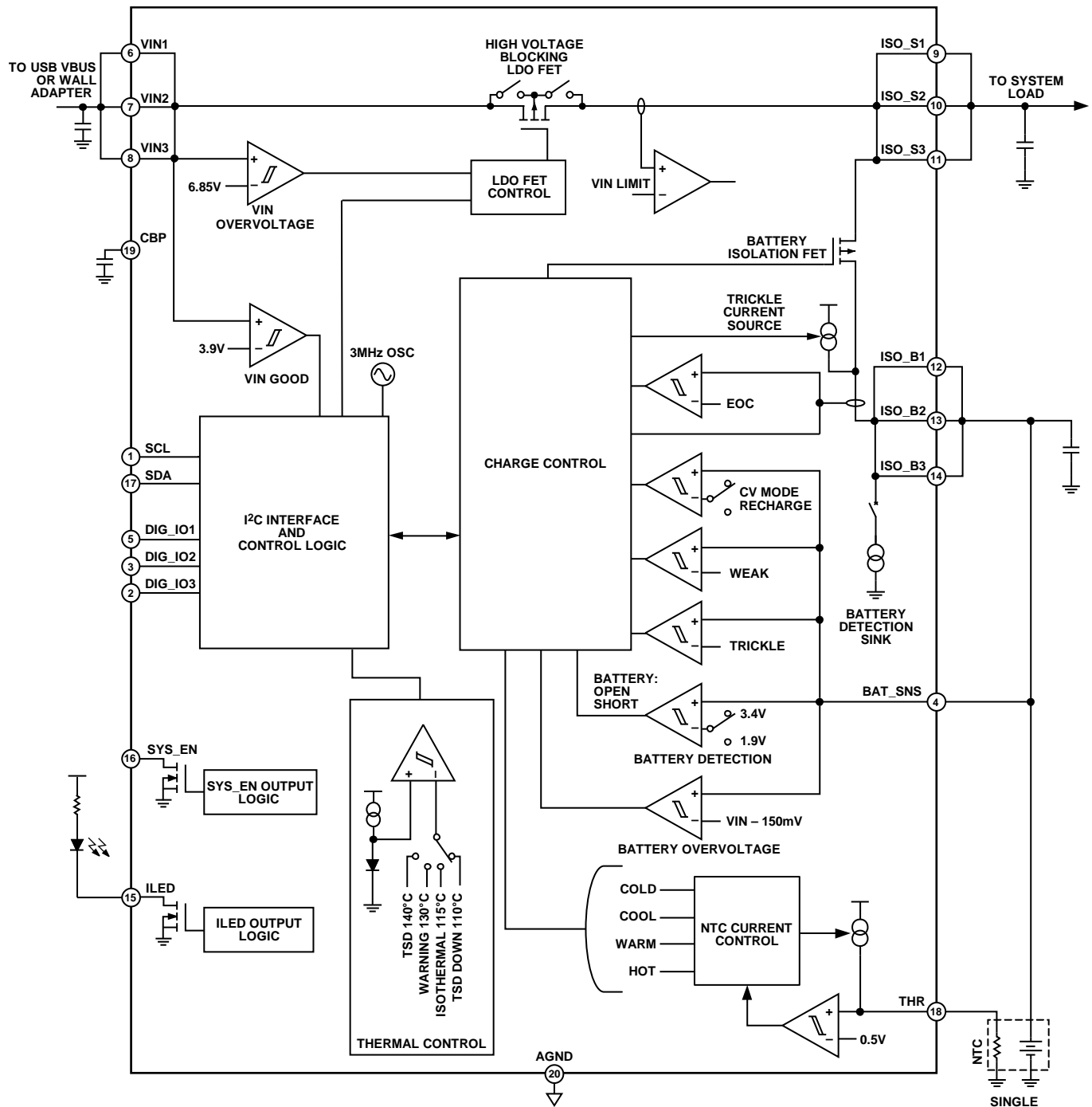
Figure 29. Block Diagram
