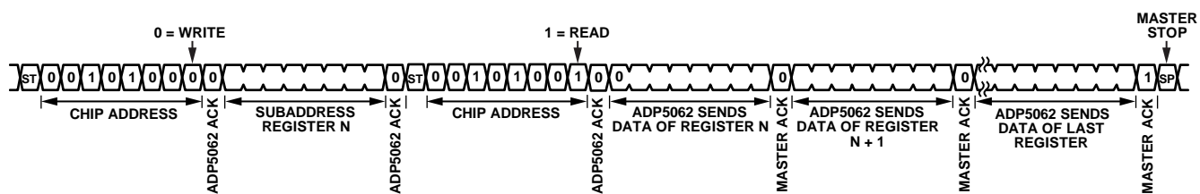
Figure 37. I 2 C Multiple Register Read Sequence
