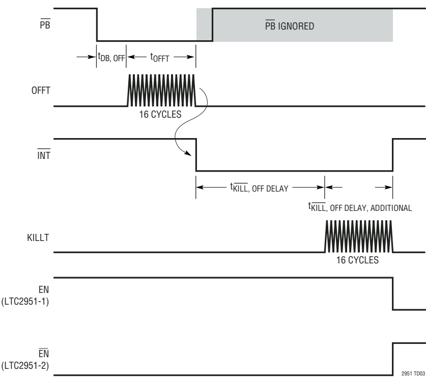
Power Off Timing, \overline{\text{KILL}} > 0.6\text{V}
