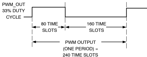
Figure 27. 33% PWM Duty Cycle Represented in Time Slots
