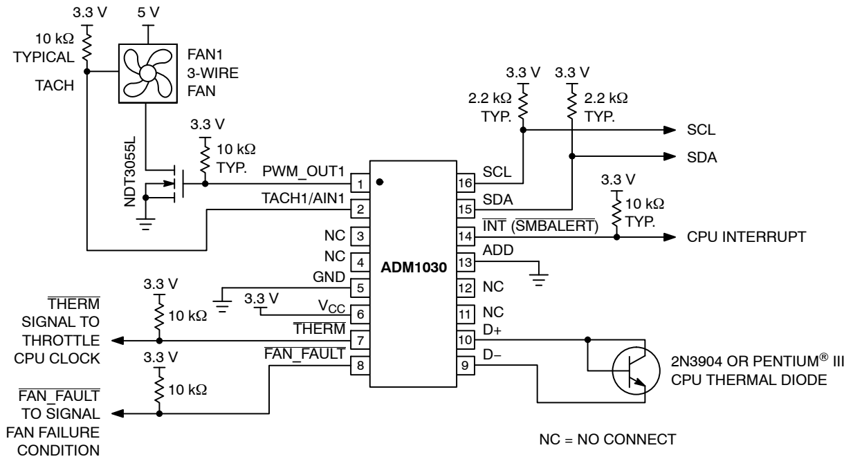
Figure 39. Typical Application Circuit
