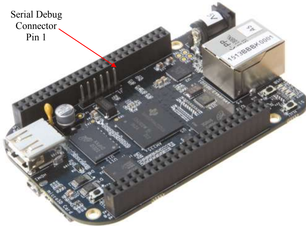
Figure 48. Serial Debug Header
