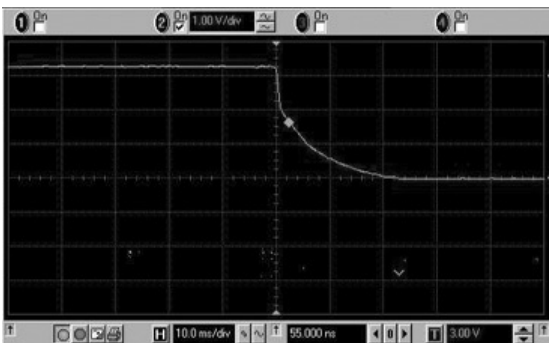
Fall Time (PWM mode): Vin = 3V; Vout = 3.3V; Iout = 2A
