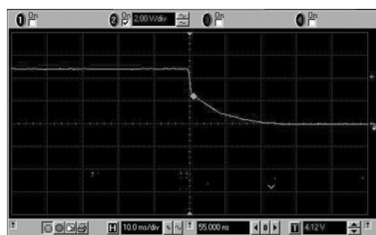
Fall Time (PWM mode): Vin = 4.5V; Vout = 5V; Iout = 2A
