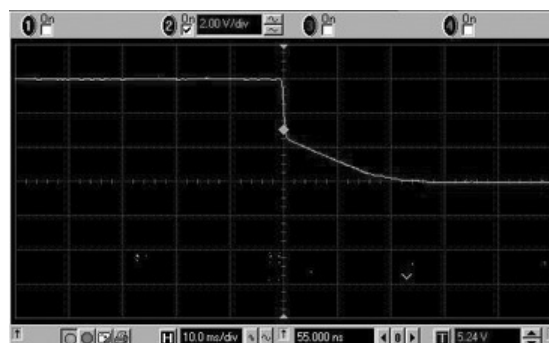
Fall Time (PWM mode): Vin = 5V; Vout = 6V; Iout = 1A
