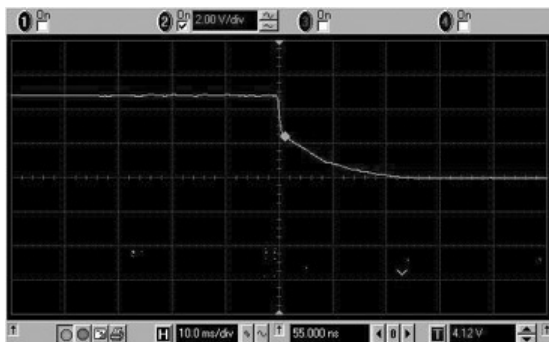
Fall Time (PWM mode): Vin = 3.5V; Vout = 5V; Iout = 2A
