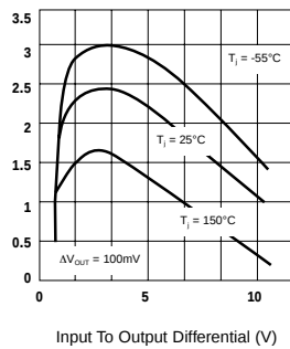
PEAK OUTPUT CURRENT
