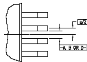
DETAIL A EVEN LEAD SIDES
