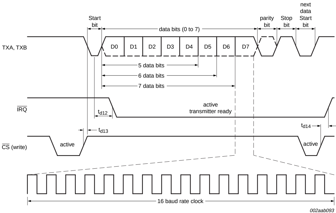
Fig 12. Transmit timing
