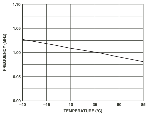
TPC 8. Oscillator Frequency vs. Temperature
