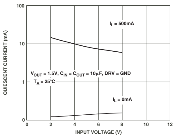
TPC 3. Quiescent Current vs. Input Voltage
