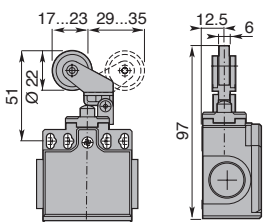
Plastic Roller on Metal Plunger
