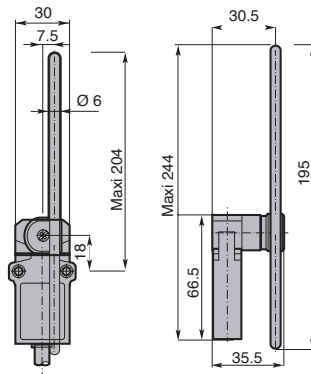
Adjustable Rod Lever
