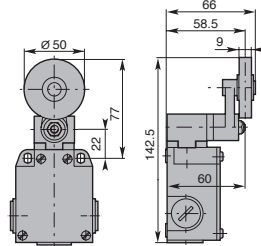
Rubber Roller Lever
