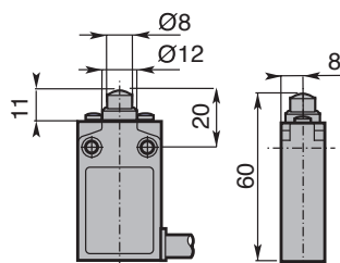
Plain Plunger
