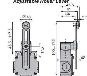
Adjustable Roller Lever
