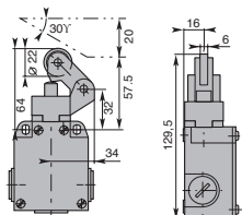
Adjustable Rubber Roller Lever
