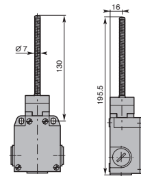
Stainless Steel Spring Multidirectional Actuator
