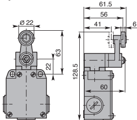
Nylon Roller Lever
