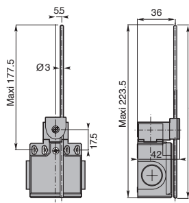
Adjustable Stainless Steel Rod Lever
