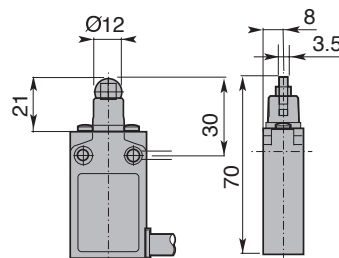
Roller Plunger
