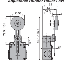
Adjustable Rubber Roller Lever
