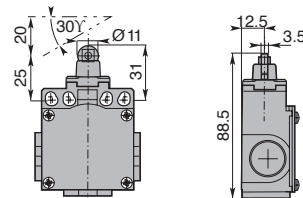
Steel Roller Plunger
