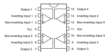
TS464CD-TS464CPT
