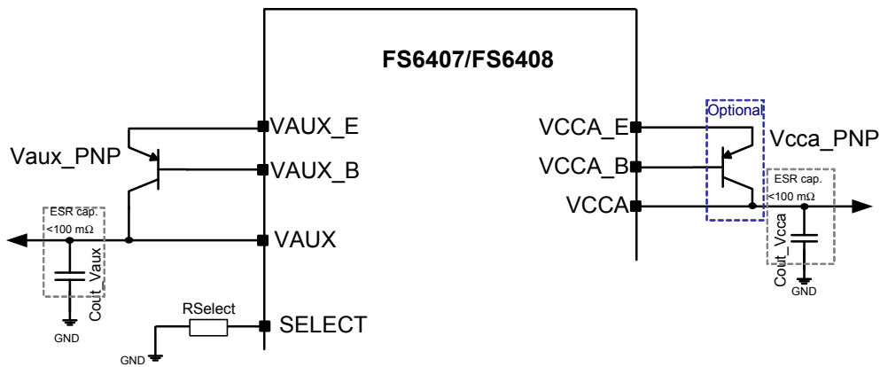
Figure 50. V_{AUX}/V_{CCA} connection
