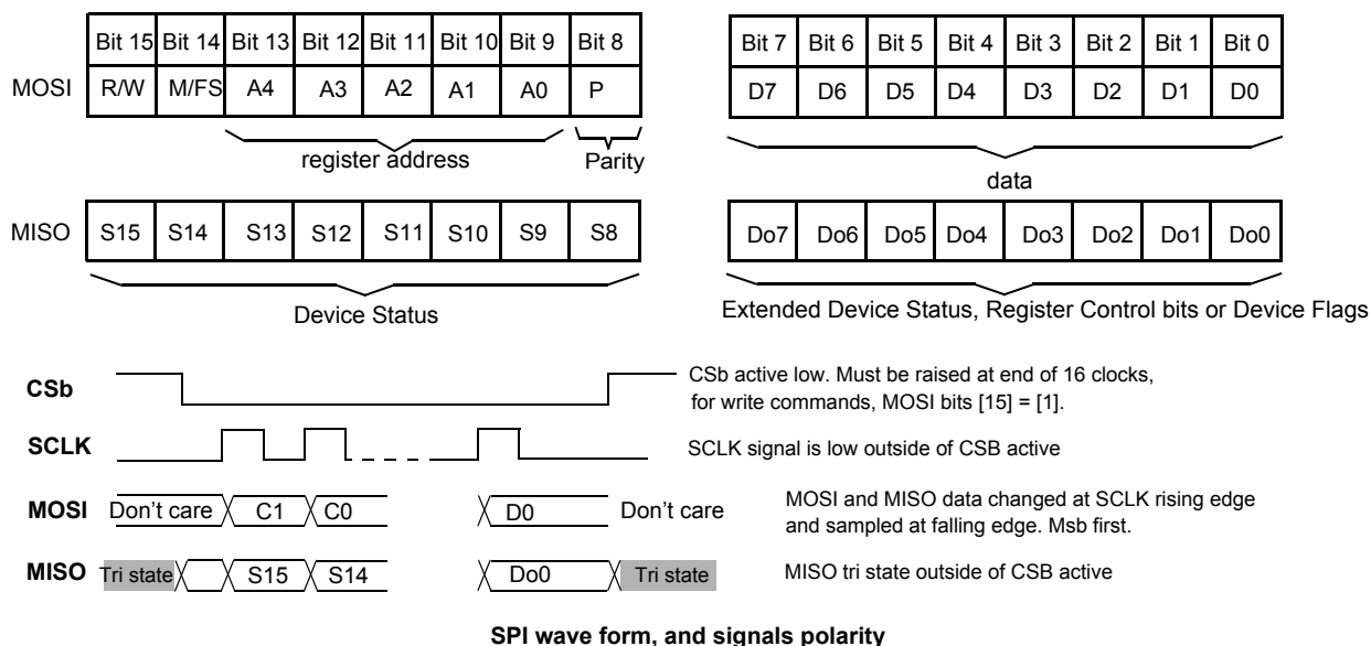
Figure 47. SPI overview
