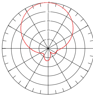
860 MHz H Plane
