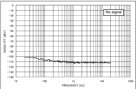
Fig.19 FFT of output noise voltage
