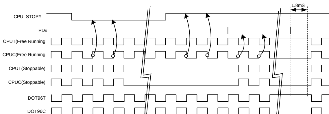
CPU_STP# = Driven, CPU_PD = Driven, DOT_PD = Driven
