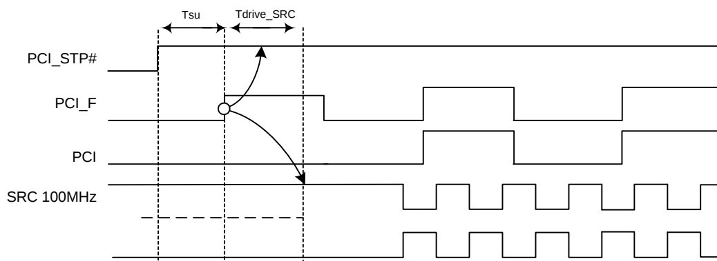
Figure 6. PCI\_STOP\# Deassertion Waveform
