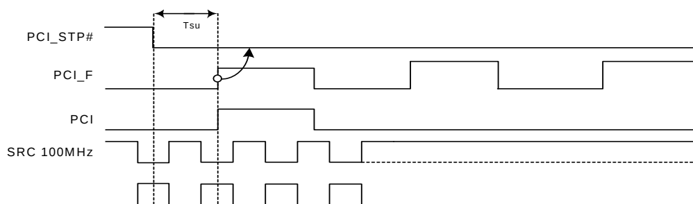
Figure 5. PCI\_STOP\# Assertion Waveform
