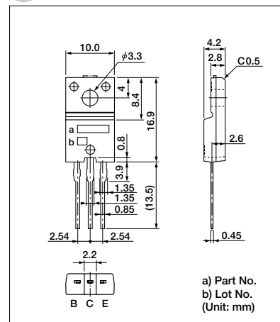
External Dimensions TO220F (full-mold)
