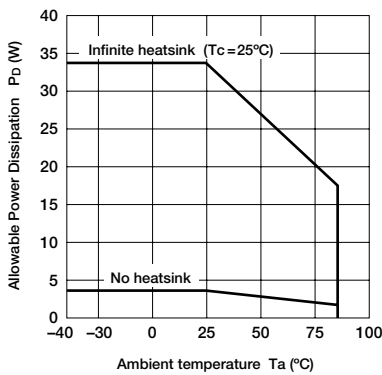
■ P_D — T_a Characteristics
