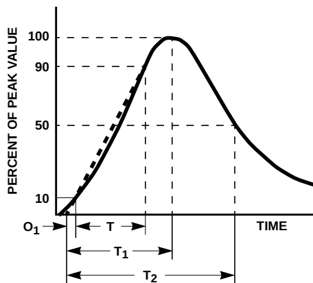
FIGURE 2. PEAK PULSE CURRENT TEST WAVEFORM
