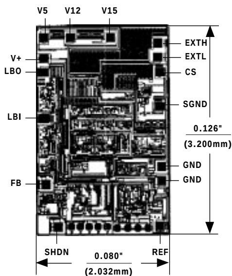
MAX773
