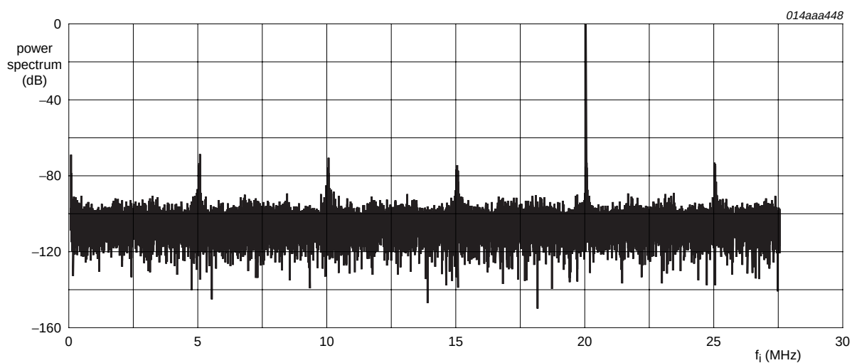
Fig 9. Single-tone; f_i = 20 MHz; f_{clk} = 55 MHz
