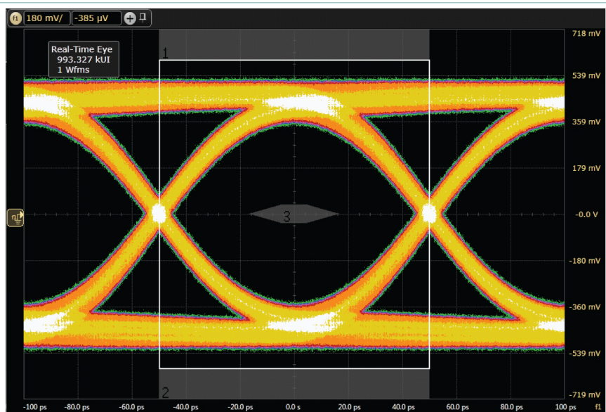
Fig. 5. USB 3.2 eye diagram 10 Gbps, test board with PCMF2USB3S; typical values
