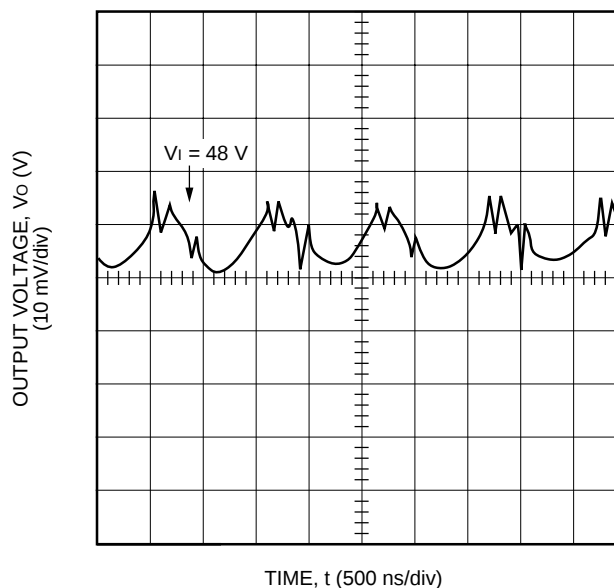
Figure 4. Typical FW300B1 Output Ripple Voltage at Room Temperature and 60 A Output
