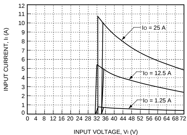
Figure 1. Typical FW300B1 Input Characteristics at Room Temperature
