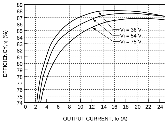
Figure 3. Typical FW300B1 Efficiency vs. Output Current at Room Temperature
