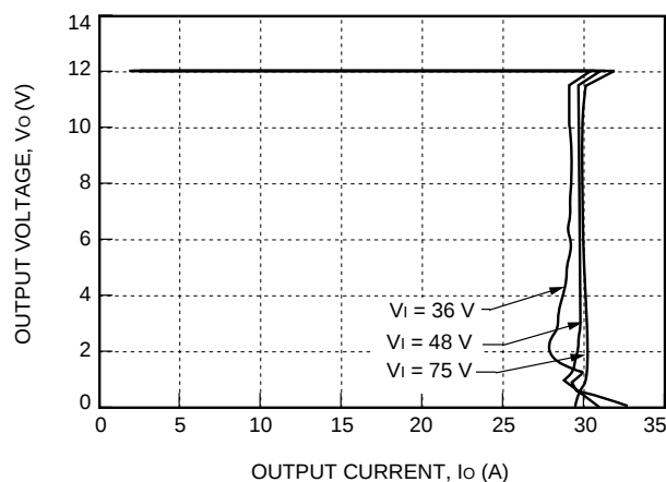
Figure 2. Typical FW300B1 Output Characteristics at Room Temperature
