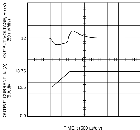
Figure 6. Typical FW300B1 Transient Response to Step Increase in Load from 50% to 75% of Full Load at Room Temperature and 48 V Input (Waveform Averaged to Eliminate Ripple Component.)
