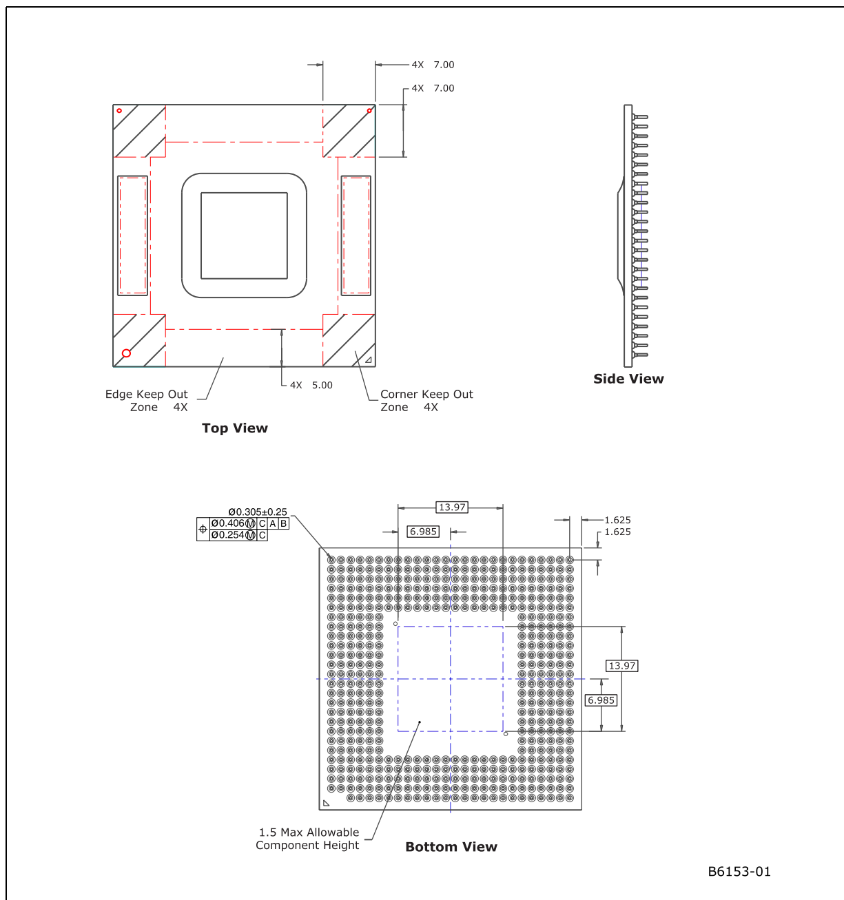
Figure 9. 2-MB Micro-FCPGA Processor Package Drawing
