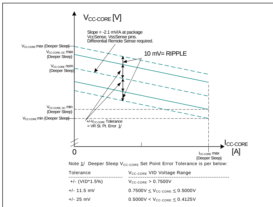
Figure 4. Deeper Sleep V_{CC} and I_{CC} Loadline for Dual-core Low Voltage and Ultra Low Voltage Processor
