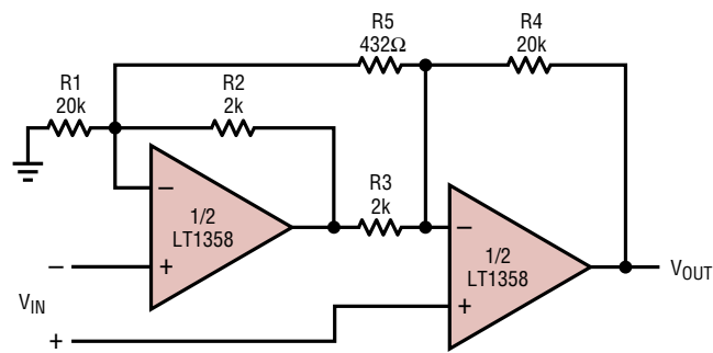
Instrumentation Amplifier
