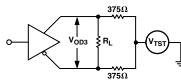
Figure 5. Driver Voltage Measurement Test Circuit 2
