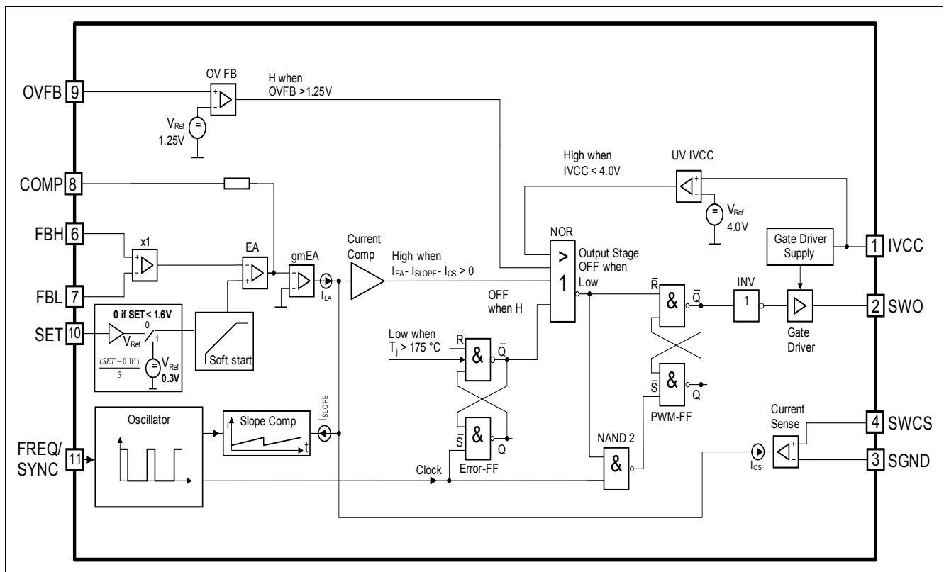
Figure 3 Switching Regulator Block Diagram
