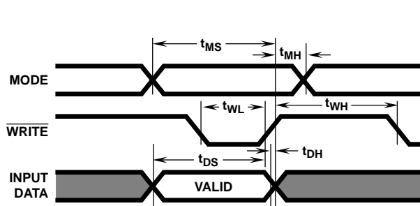
FIGURE 1. ICM7228A/B WRITE CYCLE
