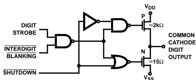
13A. DIGIT DRIVER
