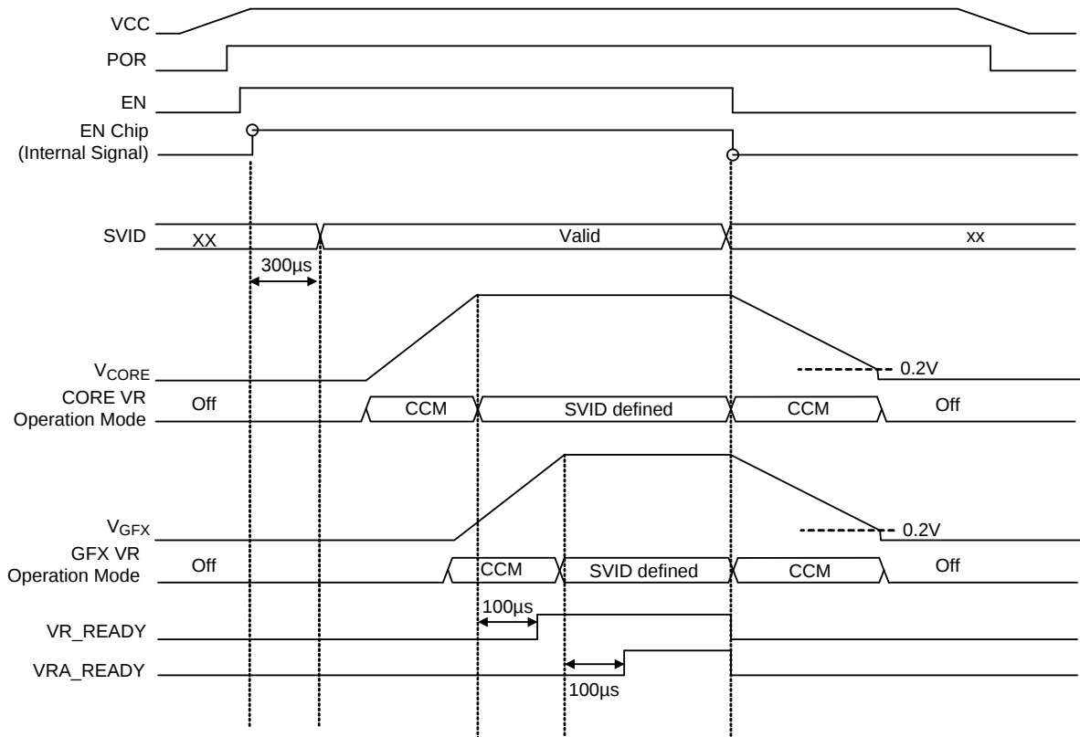
Figure 7 (a). Power sequence for RT8167B ( V_{INI\_CORE} = V_{INI\_GFX} = 0V )
