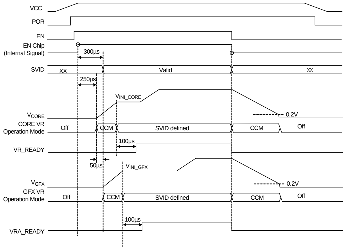
Figure 7 (b). Power sequence for RT8167B ( V_{INI\_CORE} \neq 0, V_{INI\_GFX} \neq 0V )
