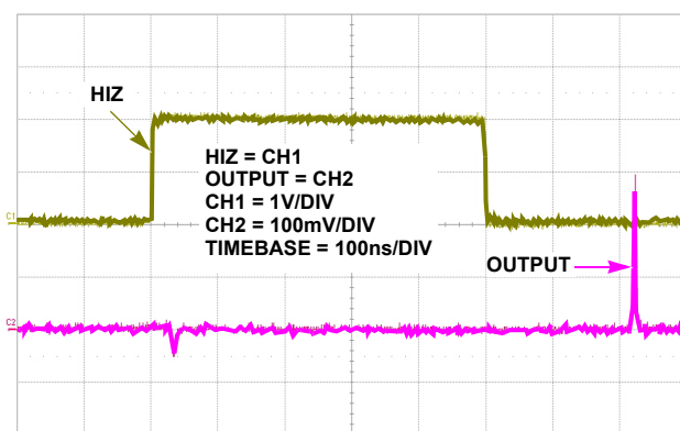
FIGURE 26. HIZ SWITCHING GLITCH, V_{IN} = 0 , GAIN = 2
