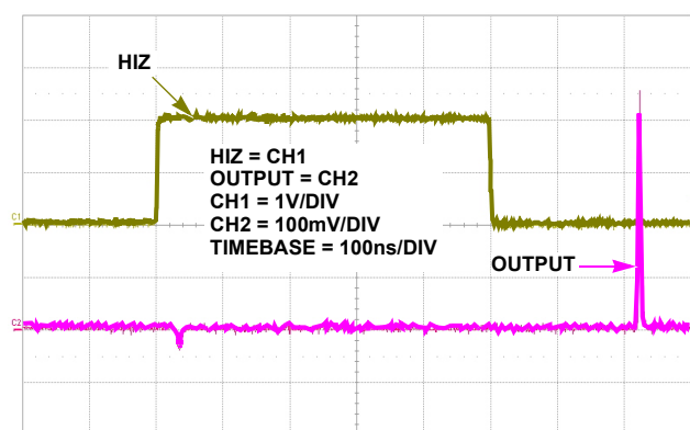
FIGURE 25. HIZ SWITCHING GLITCH, V_{IN} = 0 , GAIN = 1
