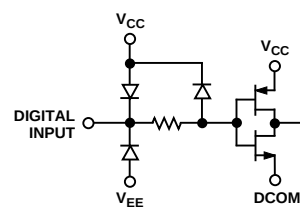
Figure 11. Equivalent Digital Input Circuit
