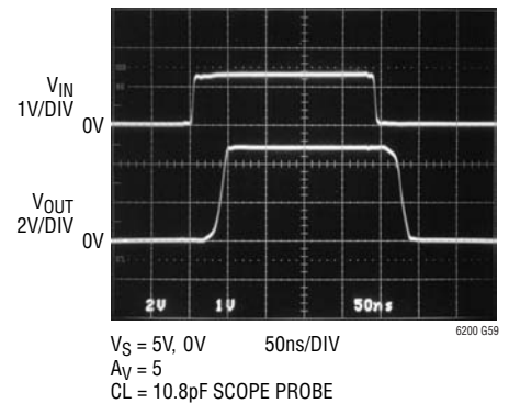
Output-Overdrive Recovery
