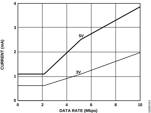
Figure 14. Typical ADuM3401W V_{DD2} Supply Current vs. Data Rate for 5 V and 3 V Operation
