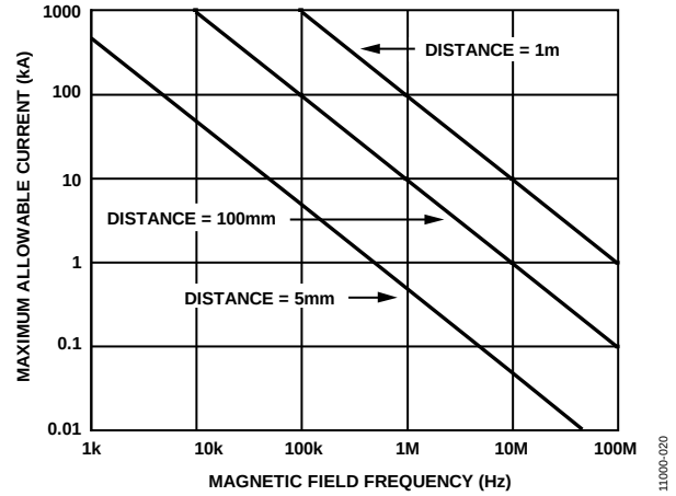
Figure 20. Maximum Allowable Current for Various Current-to- ADuM340xW Spacings
