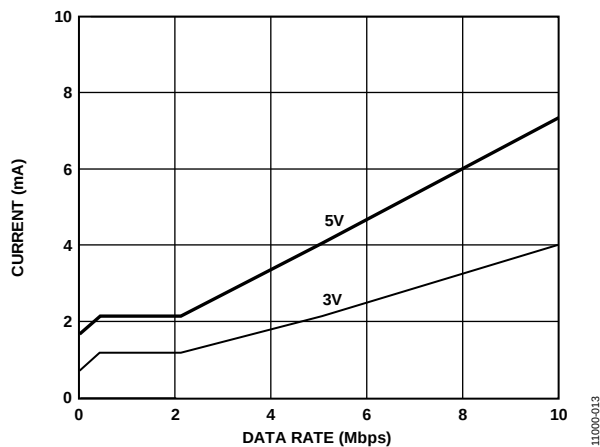
Figure 13. Typical ADuM3401W V_{DD1} Supply Current vs. Data Rate for 5 V and 3 V Operation
