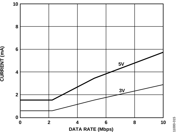
Figure 15. Typical ADuM3402W V_{DD1} or V_{DD2} Supply Current vs. Data Rate for 5 V and 3 V Operation
