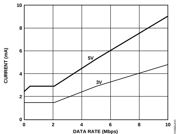
Figure 11. Typical ADuM3400W V_{DD1} Supply Current vs. Data Rate for 5 V and 3 V Operation
