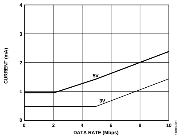
Figure 12. Typical ADuM3400W V_{DD2} Supply Current vs. Data Rate for 5 V and 3 V Operation
