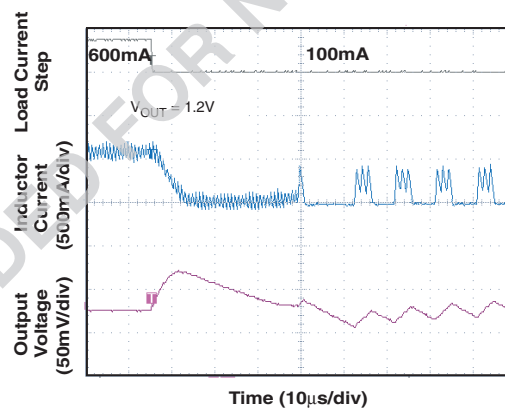
Figure 12. Load Transient Response
