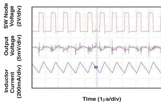
Figure 9. PWM Mode
