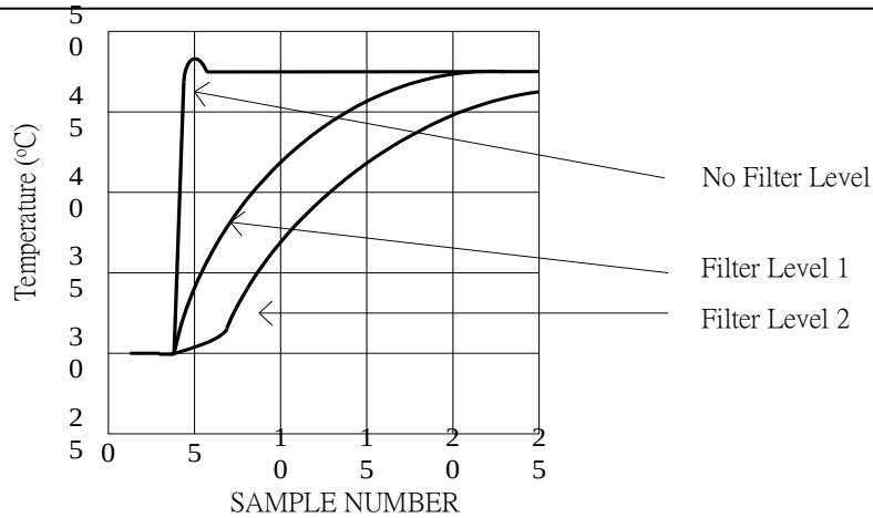
Figure 7.4.1 Step Response of reading remote temperature
