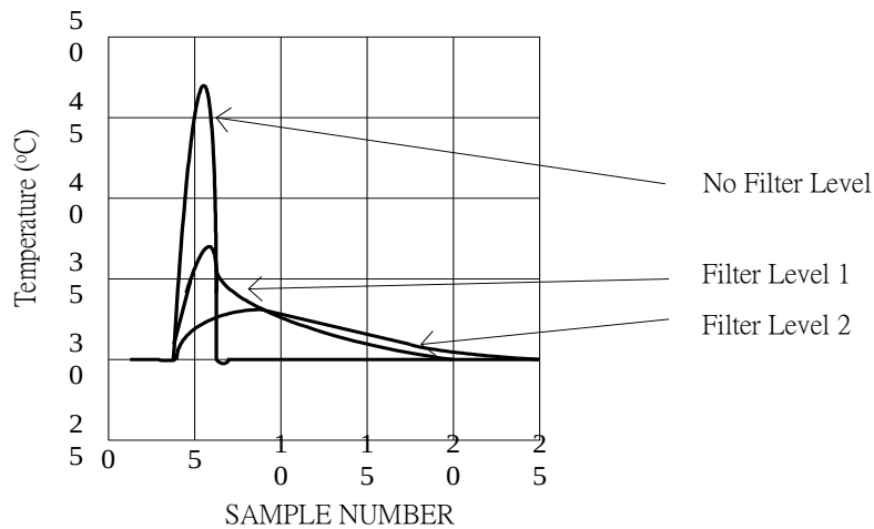
Figure 7.4.2 Impulse Response of reading remote temperature
