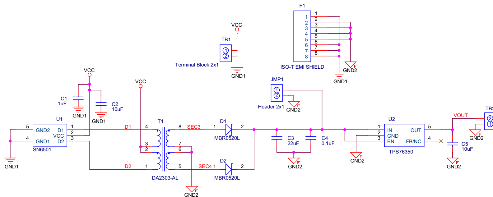
Figure 2. SN6501-5EVM Schematic
