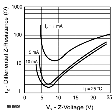
Figure 10. Differential Z-Resistance vs. Z-Voltage
