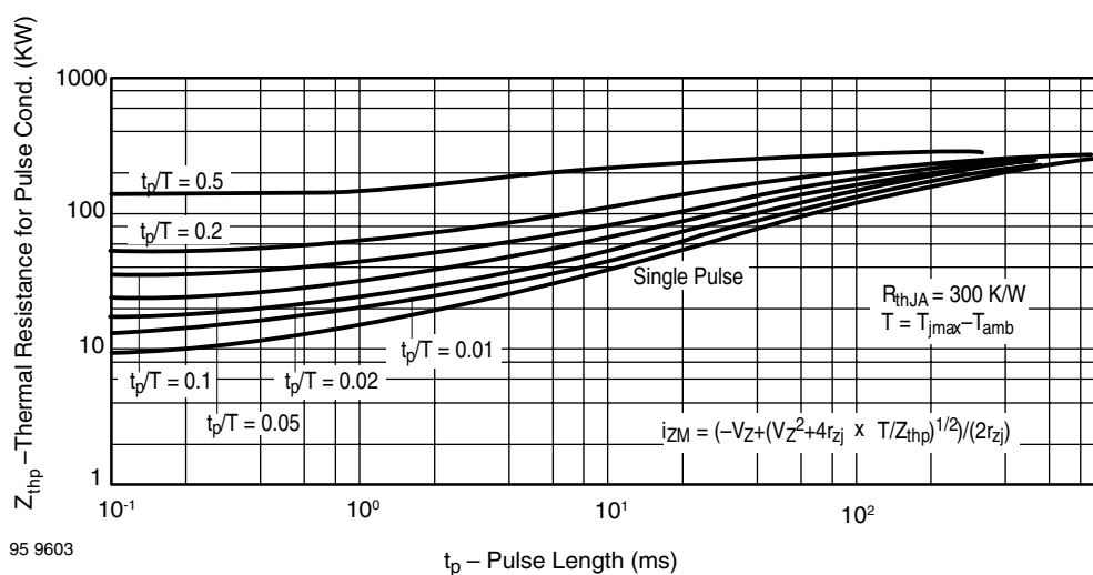
Figure 11. Thermal Response
