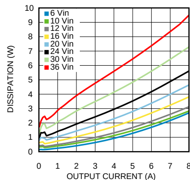
Figure 8. Dissipation 1.8-V Output at 25°C
