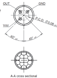
A-A cross sectional
