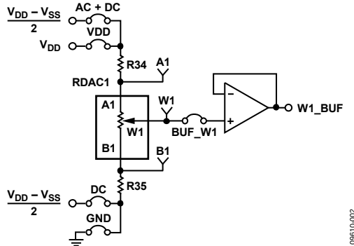
Figure 2. DAC
