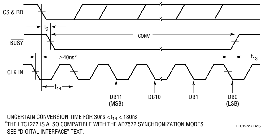
Figure 13. \overline{\text{RD}} and CLK IN for Synchronous Operation
