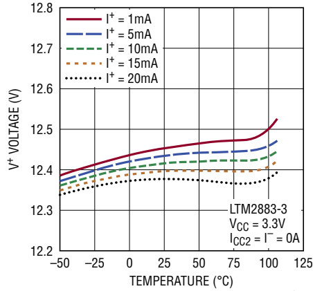
V^+ Load Regulation vs Temperature
