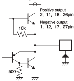
Driver output
