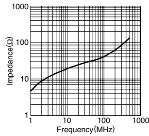
HF70SH13X1.3X12
