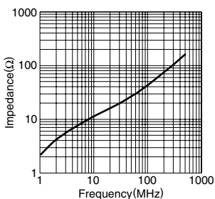
HF70SH40X1.3X8
