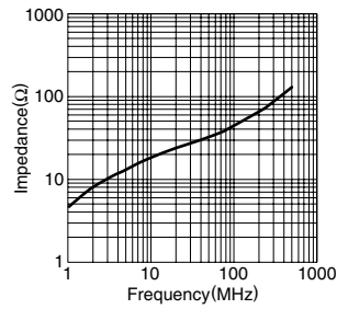
HF70SH13X0.7X12
