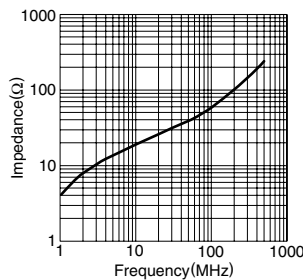
HF70SH35X1.3X12
