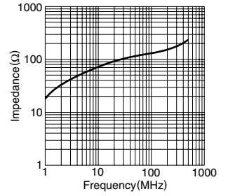
HF70SH10X0.6X5
