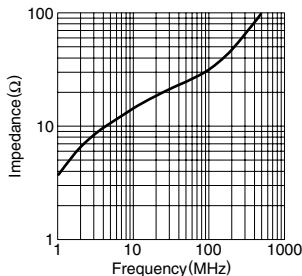
HF70SH11X0.7X8
