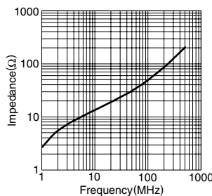
HF70SH46X1.9X10
