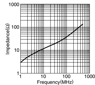
HF70SH20X0.7X8
