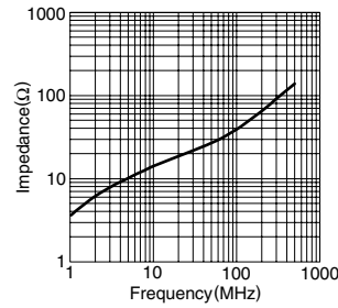
HF70SH15X0.7X10
