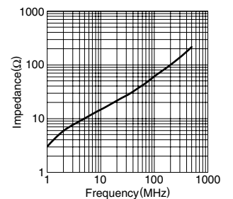
HF70SH41X0.8X12
