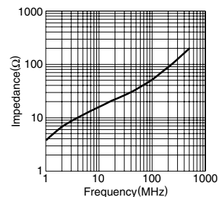
HF70SH20X0.7X12
