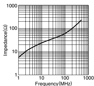
HF70SH40X2X12
