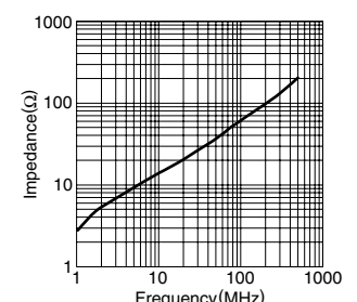
HF70SH52X1X12
