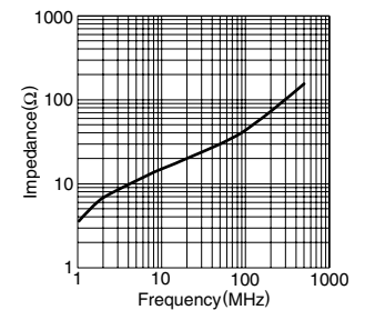
HF70SH20X0.9X12
