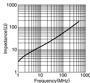
HF70SH42X0.9X12
