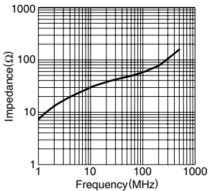
HF70SH12X0.9X12
