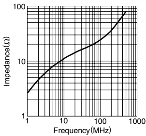
HF70SH9X0.7X10
