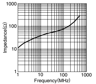
HF70SH18.8X1.1X15
