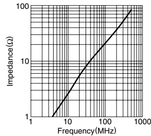
HF70SH13X0.7X3A
