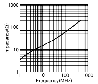
HF70SH35X0.8X12
