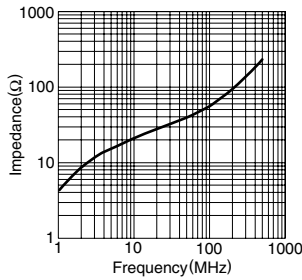
HF70SH27X1.3X10
