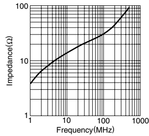
HF70SH10X1X6
