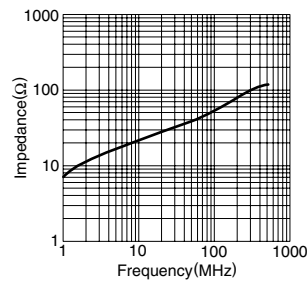
HF70SH21X0.8X12
