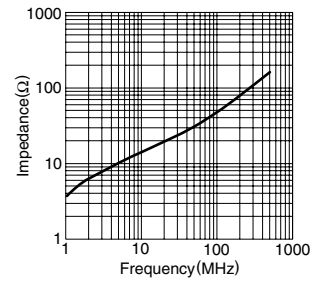
HF70SH25X0.7X10
