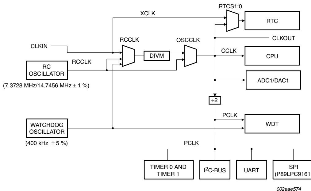
Fig 10. Block diagram of oscillator control
