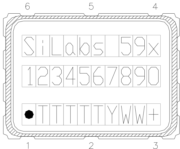
Figure 6. Mark Specification
