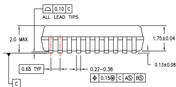
DIMENSIONS ARE IN MILLIMETERS
