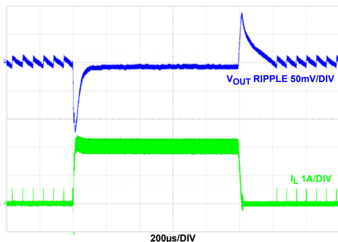
FIGURE 45. LOAD TRANSIENT F_{SW} = 2\text{MHz} , V_{IN} = 5\text{V} , \text{MODE} = \text{PFM} , T_A = +25^\circ\text{C}
