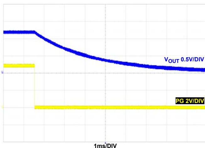
FIGURE 52. OVER-TEMPERATURE PROTECTION F_{SW} = 2\text{MHz} , V_{IN} = 5\text{V} , MODE = PWM, T_A = +163^\circ\text{C}
