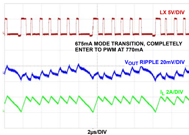
FIGURE 49. PFM TO PWM TRANSITION F_{SW} = 2\text{MHz} , V_{IN} = 5\text{V} , \text{MODE} = \text{PFM} , T_A = +25^\circ\text{C}
