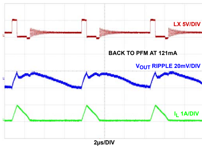
FIGURE 50. PWM TO PFM TRANSITION F_{SW} = 2\text{MHz} , V_{IN} = 5\text{V} , \text{MODE} = \text{PWM} , T_A = +25^\circ\text{C}
