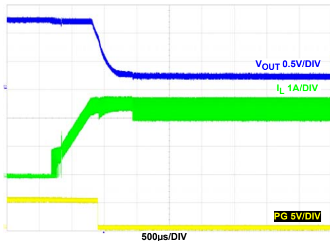
FIGURE 48. OVERCURRENT PROTECTION F_{SW} = 2\text{MHz} , V_{IN} = 5\text{V} , \text{MODE} = \text{PWM} , T_A = +25^\circ\text{C}
