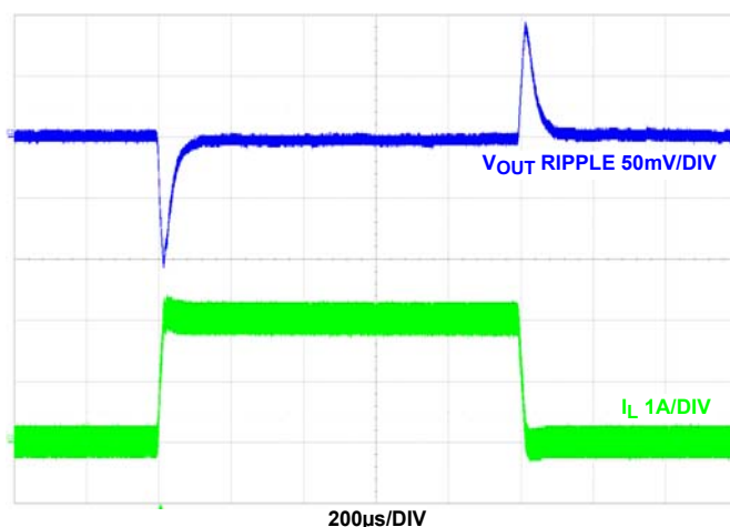
FIGURE 46. LOAD TRANSIENT F_{SW} = 2\text{MHz} , V_{IN} = 5\text{V} , \text{MODE} = \text{PWM} , T_A = +25^\circ\text{C}
