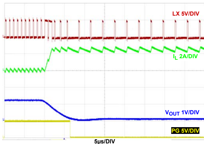
FIGURE 47. OUTPUT SHORT-CIRCUIT F_{SW} = 2\text{MHz} , V_{IN} = 5\text{V} , \text{MODE} = \text{PFM} , T_A = +25^\circ\text{C}
