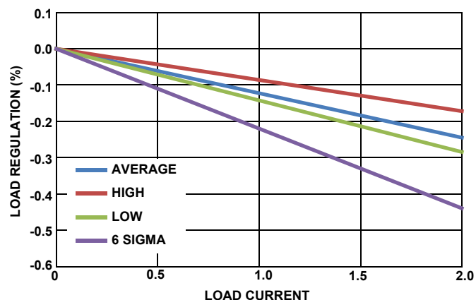
FIGURE 12. LOAD REGULATION, T_A = +105^\circ\text{C} , 2.7\text{V}_{IN} , 0.6\text{V}_{OUT} , 1\text{MHz}
