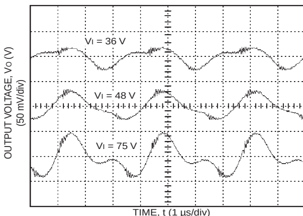
Figure 15. Output Ripple Voltage ( I_O = I_{O, \text{max}} ).
